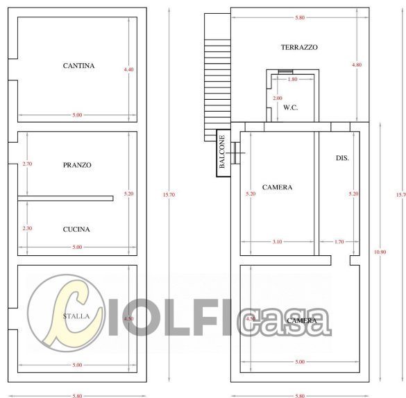
PIANO TERRA H= 3.20 ml
